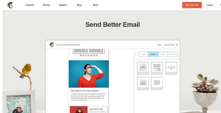
Gambar 5.15 www.mailchimp.com
