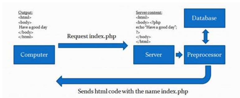
Gambar 2.13 Website Dinamis
