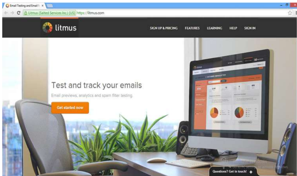
Gambar 5.24 https://litmus.com/
