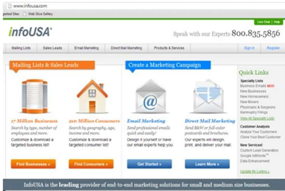
Gambar 5.10 http://www.infousa.com/
