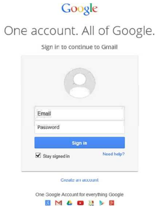
Gambar 5.35 Sign in.
