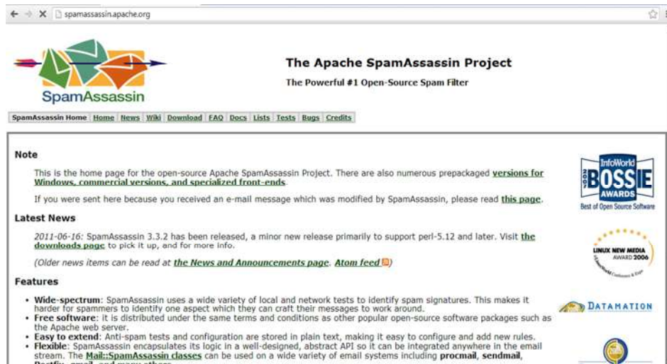
Gambar 5.27 http://spamassassin.apache.org .
