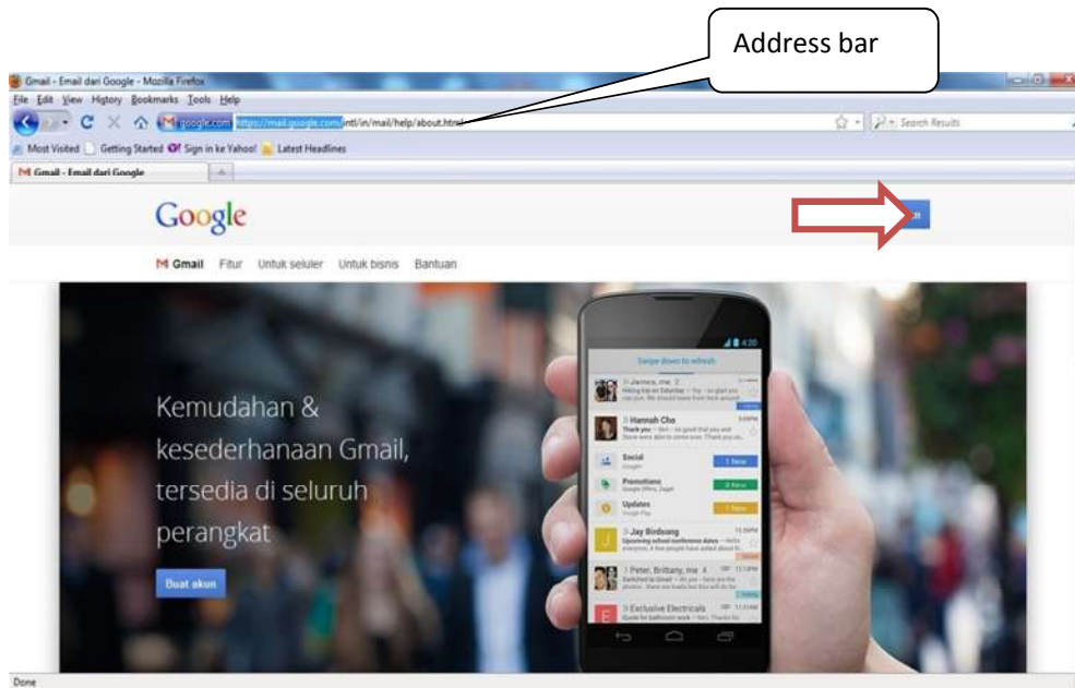
Gambar 5.32 Webmail Gmail
