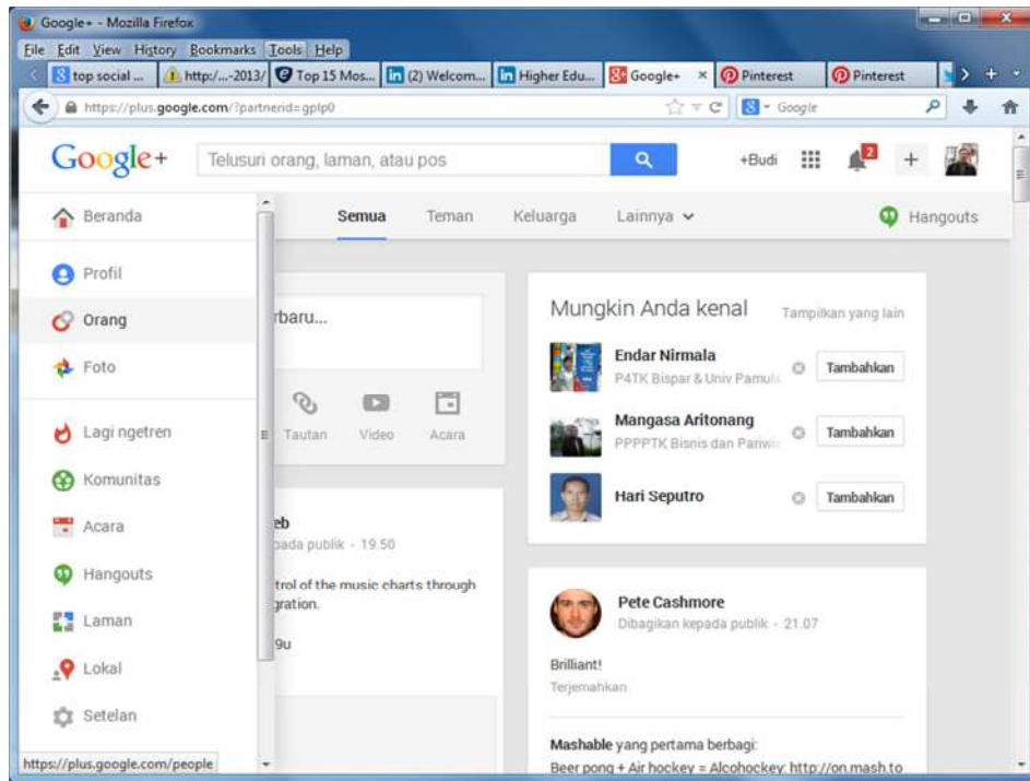
Gambar 4.4 https://plus.google.com
