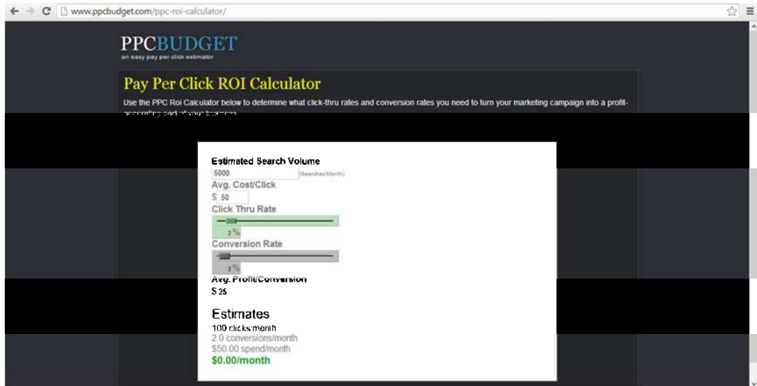
Gambar 6.8 http://www.ppcbudget.com
