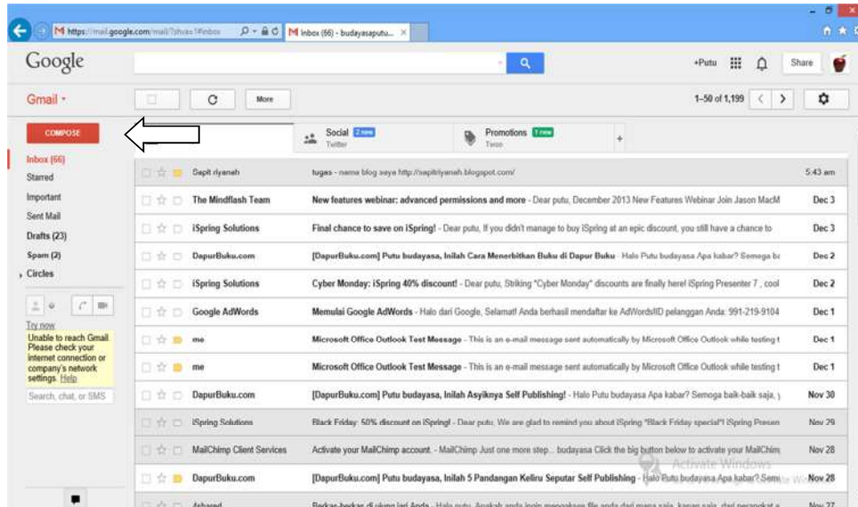
Gambar 5.36 Webmail Gmail
