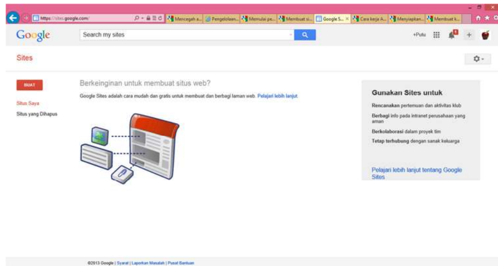
Gambar 6.21 www.google.com/sites
