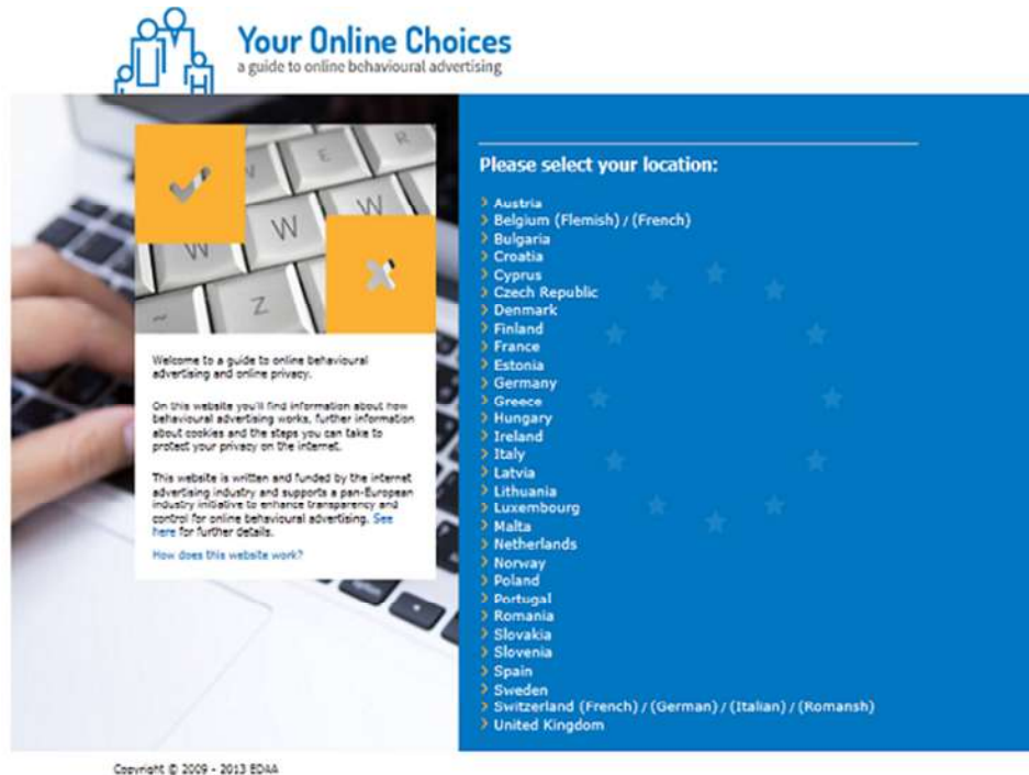
Gambar 5.9 http://www.youronlinechoices.com/
