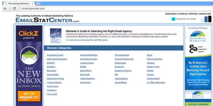
Gambar 5.25 http://emailstatcenter.com
