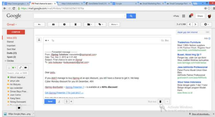
Gambar 5.44 Tampilan Forward.
