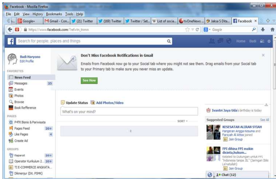
Gambar 4.1 https://www.facebook.com
