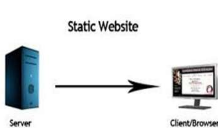
Gambar 2.12 Website Statis
