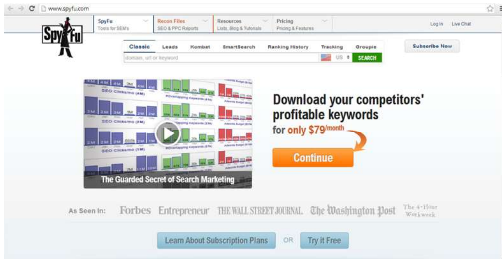
Gambar 6.9 www.spyfu.com
