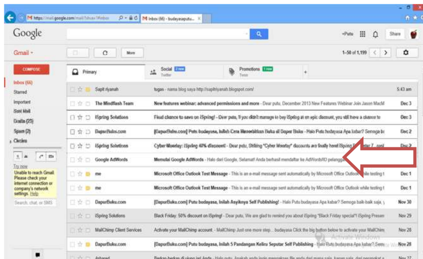
Gambar 5.40 Check mail.
